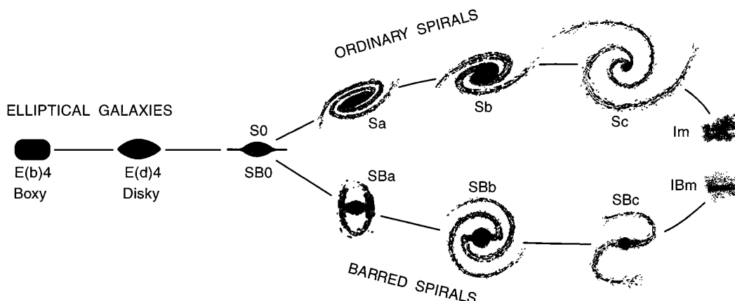
FIG. 1.—Proposed morphological classification scheme for elliptical galaxies. Ellipticals are illustrated edge-on and at ellipticity \epsilon \approx 0.4 . The connection between boxy and disk-like ellipticals may not be continuous (see § 4). This figure is based on the tuning-fork diagram of Hubble (1936). We make three additional modifications: we illustrate the two-component nature of S0 galaxies and label them as barred or unbarred, we call unbarred spirals “ordinary” rather than “normal” (de Vaucouleurs 1959), and we add Magellanic irregulars.
