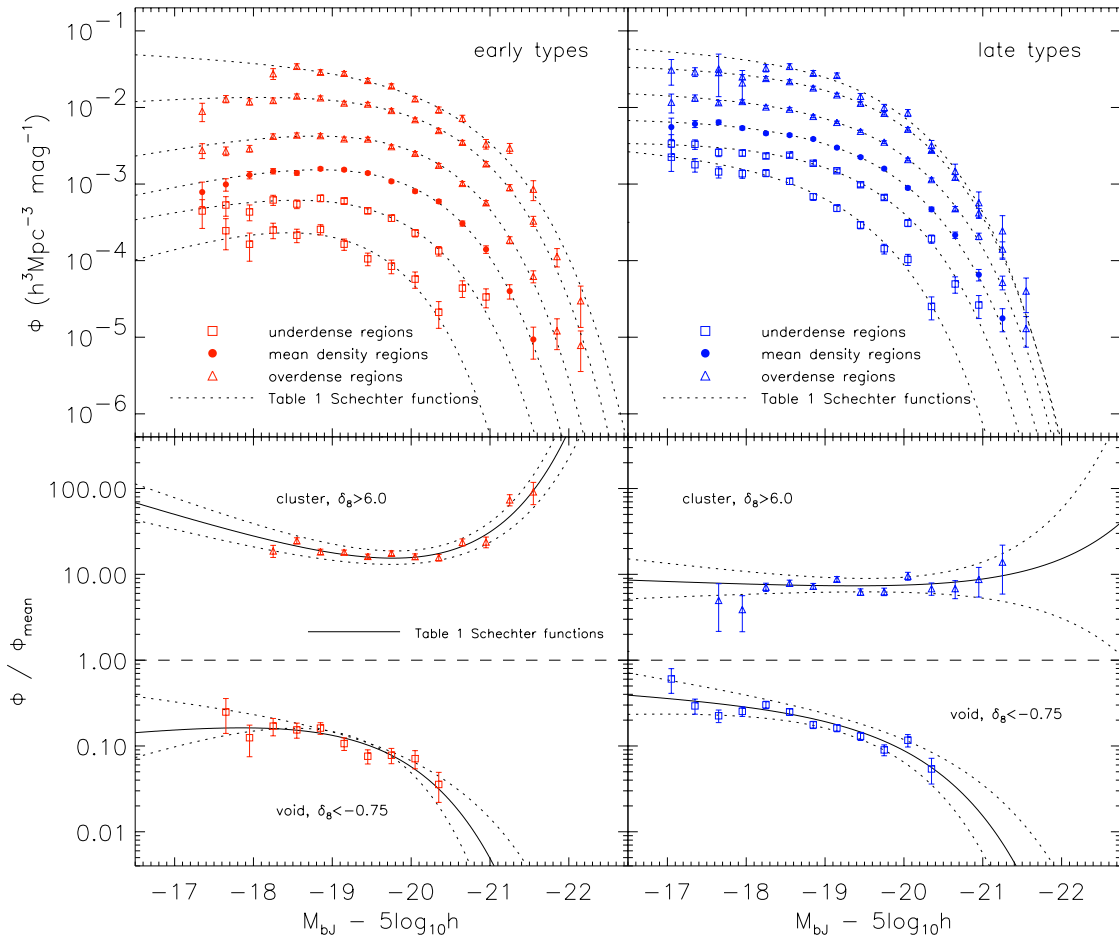
Figure 4. Comparing both the (top) absolute and (bottom) relative distributions of (left) early-type galaxies in various density environments, and (right) late-type galaxies in various density environments. In the bottom panels the luminosity functions have again been normalized to the mean (each to their respective type) as in Fig. 3 (note that the shape of the mean for each type is very similar to that shown in Fig. 1). Here the solid lines and bounding dotted lines show the appropriate Table 1 Schechter functions normalized to the mean Schechter function and 1\sigma uncertainty.
